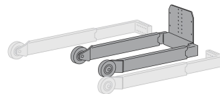
Item no. OPT0487 MD adjustable support structure - model B
