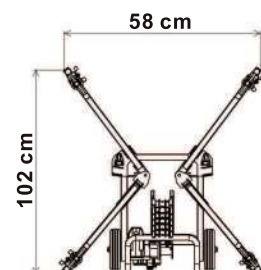
Adjustable Leg - 2
